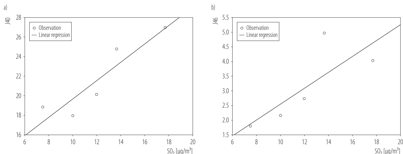
Figure 4. A dependence scatter plot representing 2 variables, \text{SO}_2 and the incidence rate of selected respiratory diseases, in region 1 of the Silesian Voivodship, for the years 2012–2017: a) bronchitis, not specified as acute or chronic (J40) and b) status asthmaticus/acute severe asthma (J46)
