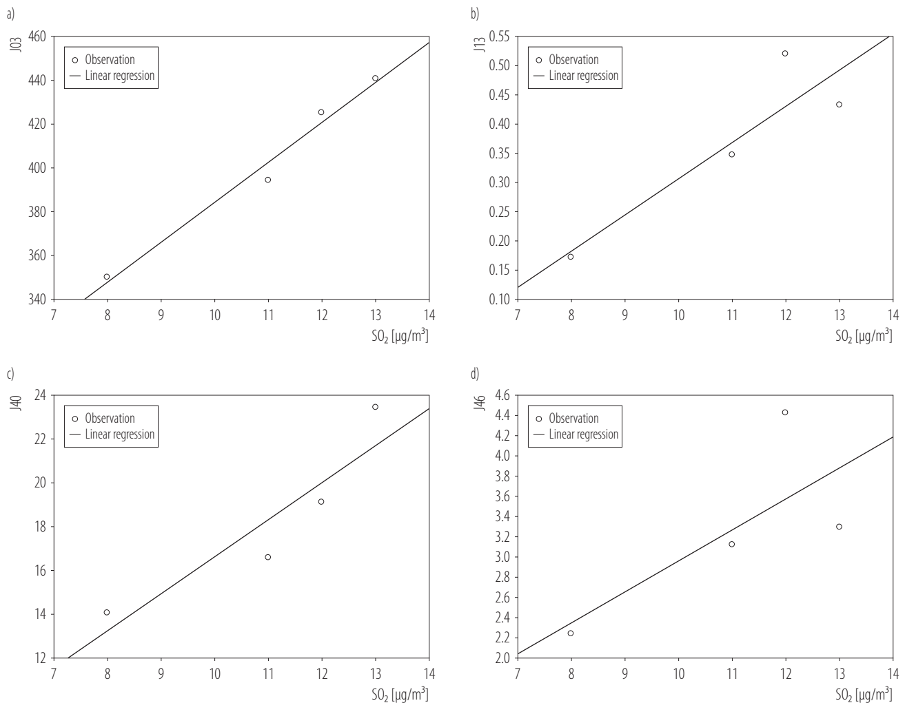
Figure 3. A dependence scatter plot representing 2 variables, \text{SO}_2 and the incidence rate of selected respiratory diseases, in region 7 of the Silesian Voivodship, for the years 2012–2017: a) acute tonsillitis (J03), b) pneumonia due to Streptococcus pneumoniae (J13), c) bronchitis, not specified as acute or chronic (J40), and d) status asthmaticus/acute severe asthma (J46)
