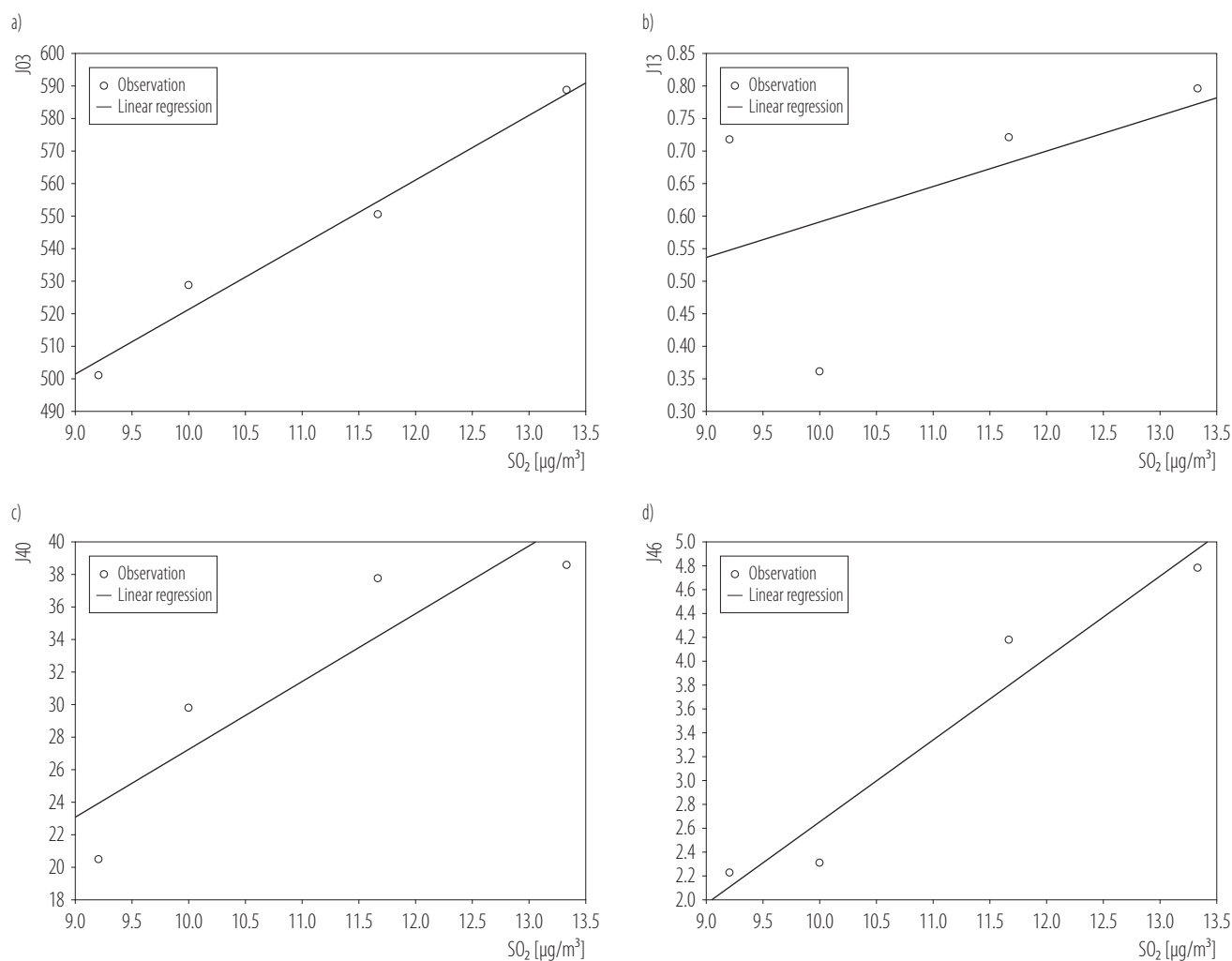
Figure 2. A dependence scatter plot representing 2 variables, \text{SO}_2 and the incidence rate of selected respiratory diseases, in region 8 of the Silesian Voivodship, for the years 2012–2017: a) acute tonsillitis (J03), b) pneumonia due to Streptococcus pneumoniae (J13), c) bronchitis, not specified as acute or chronic (J40), and d) status asthmaticus/acute severe asthma (J46)
